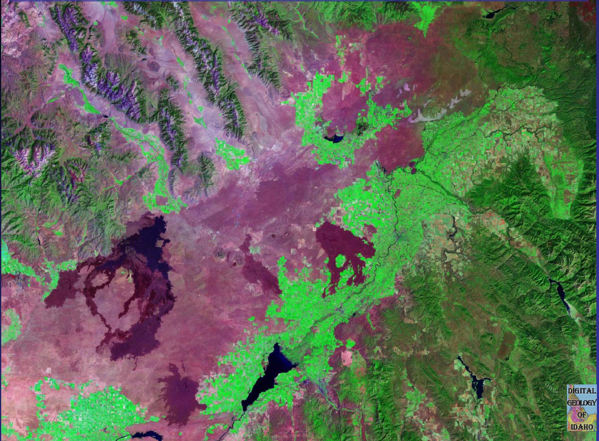
False color satellite image of eastern Idaho. Craters of the Moon at left. Lost River Valley to north. American Falls Reservoir in lower center
