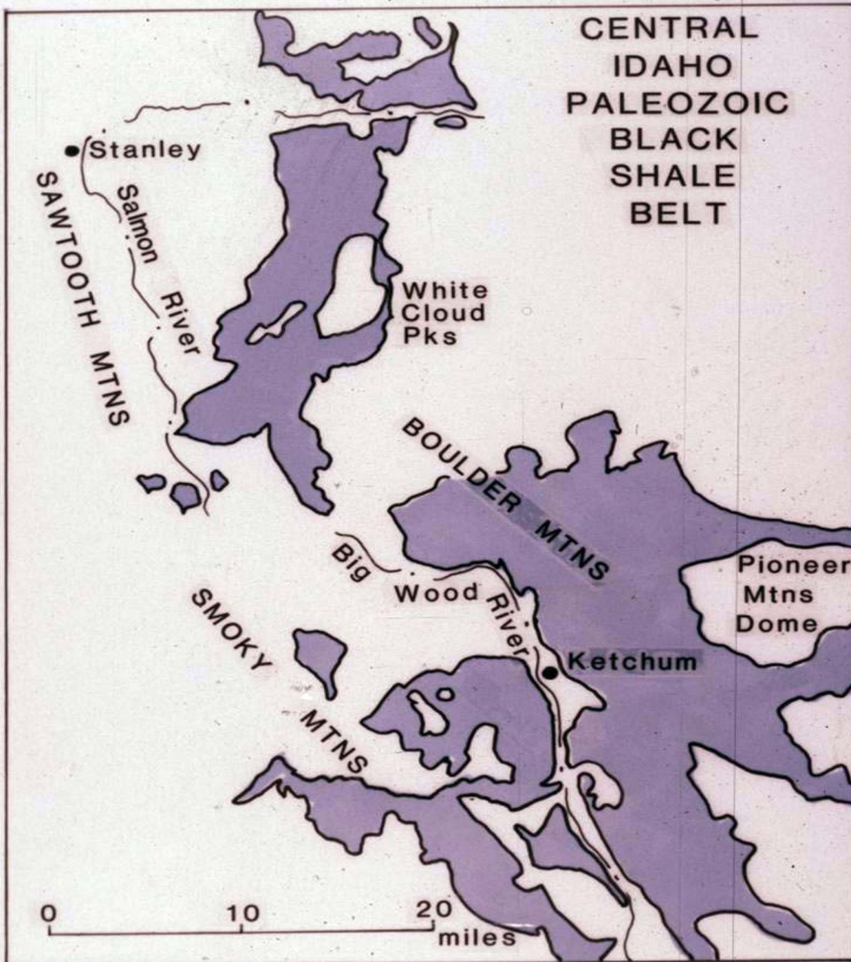
HALL, 1985, USGS Bull. 1658-J
