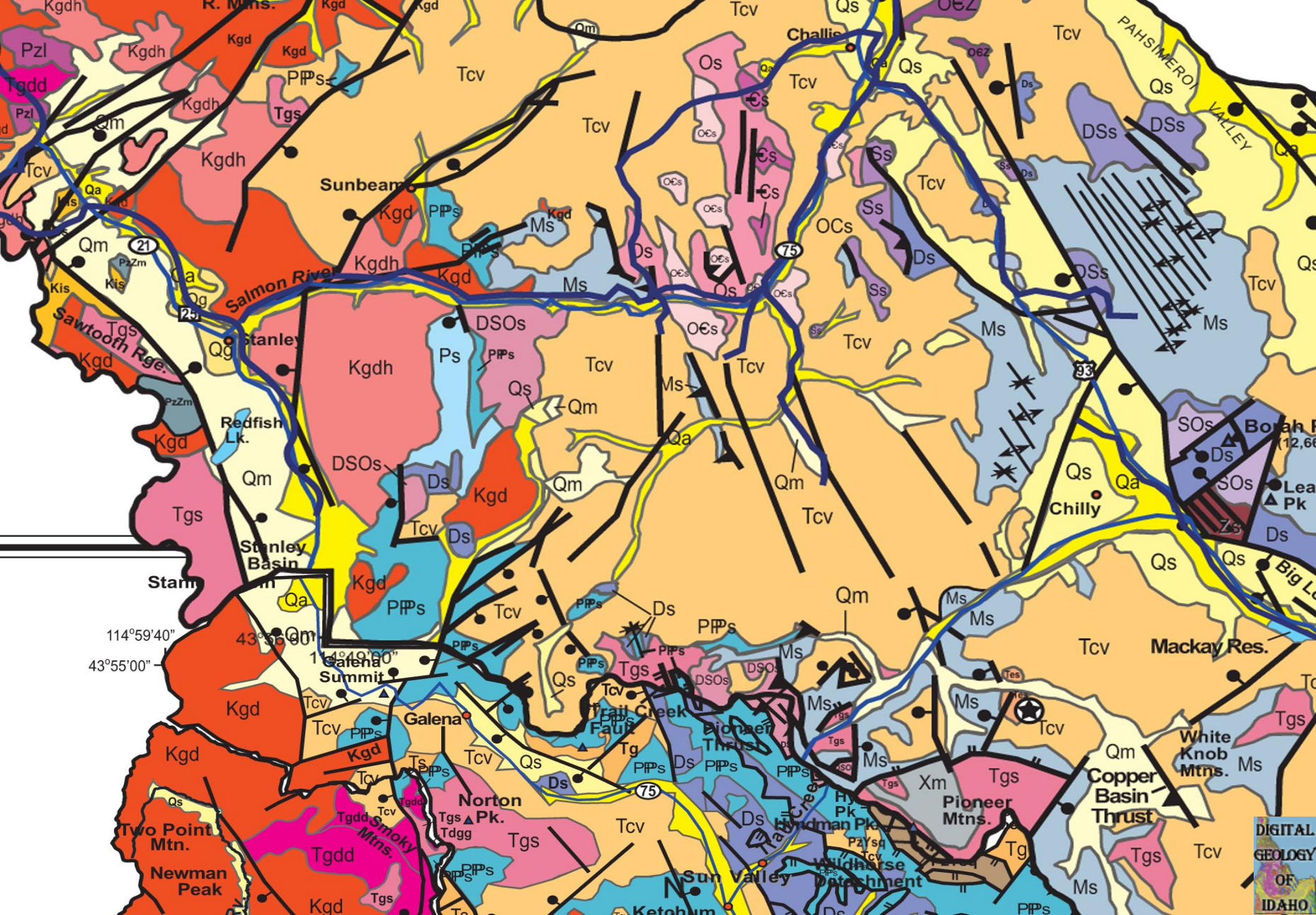
Geologic map of parts of Blaine and Custer Counties Shows cross section from Batholith east through core complex to thrust belt.
