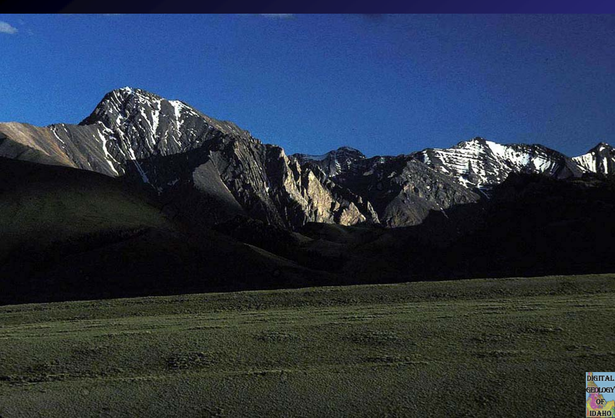
Upper Pahsimeroi view to south, east side of Lost River Range. Mt. Breitenbach on left. Folded Mississippian carbonate rocks.
